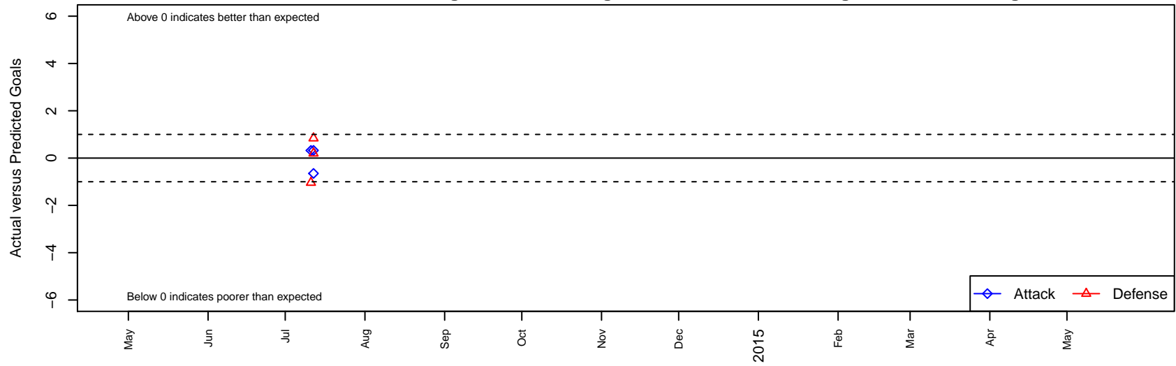
Highline Premier –Unk B01 Dots are actual minus expected GF (blue circles) and GA (red triangles). Blue line is smoothed change in attack strength. Red is smoothed change in defense strength.
